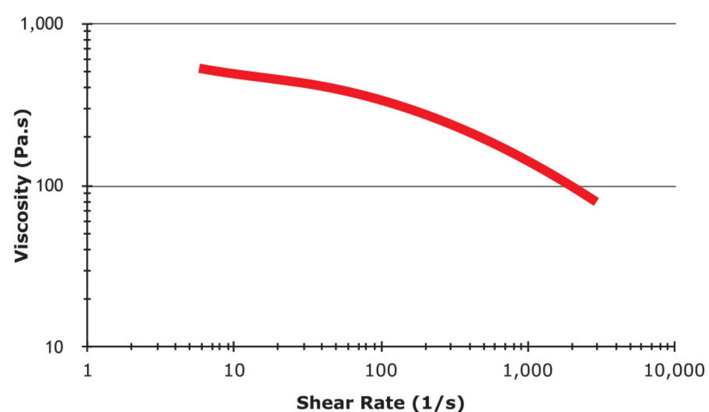
Shear-Viscosity @ 190 °C
